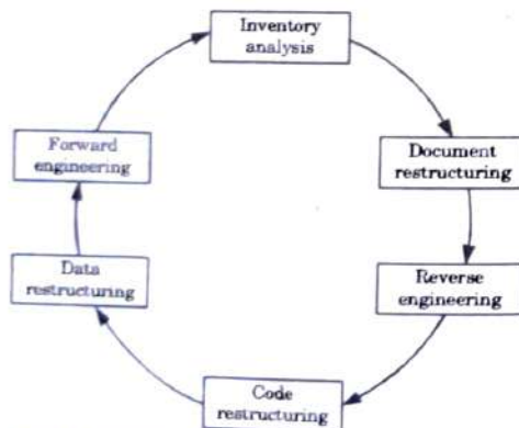
Fig. 5.8.1. Software re-engineering process model.
