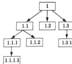
Fig. 4.5.1. Top-down integration.
