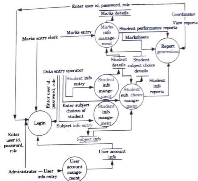
Fig. 2.20.2. Level 1 DFD of result management system.
