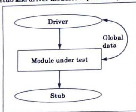
Fig. 4.15.3. Unit testing with the help of driver and stub modules.
