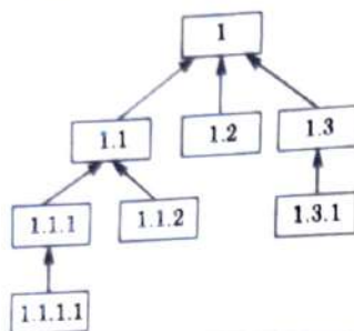
Fig. 4.5.2. Bottom-up integration testing.
