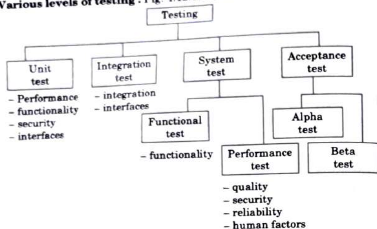
Fig. 4.12.1. Levels of testing.
