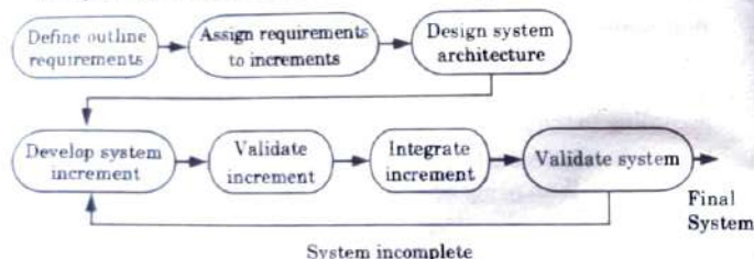
Fig. 1.21.1. Iterative enhancement model.
