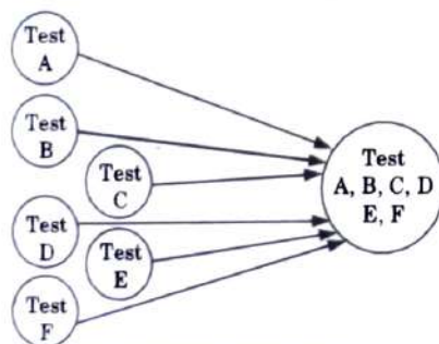
Fig. 4.5.3. Big-bang testing.
