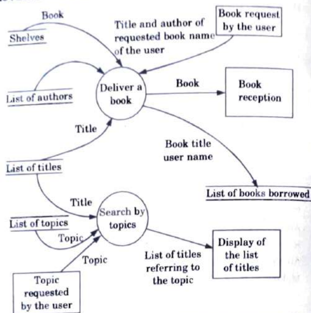
Fig. 2.10.1. A DFD describing a simplified library information system.
