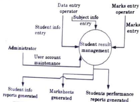
Fig. 2.20.1. 0-Level DFD or context diagram of result management system.
