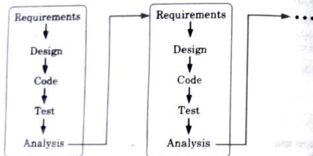
Fig. 5.3.2. Iterative enhancement model.
